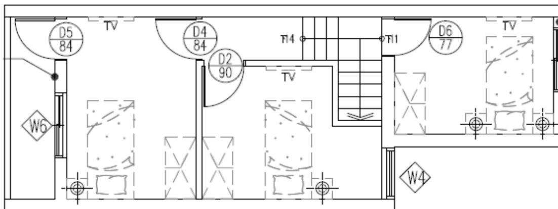
2/F floor plan of Baofu Road dormitory (after the upgrade)
