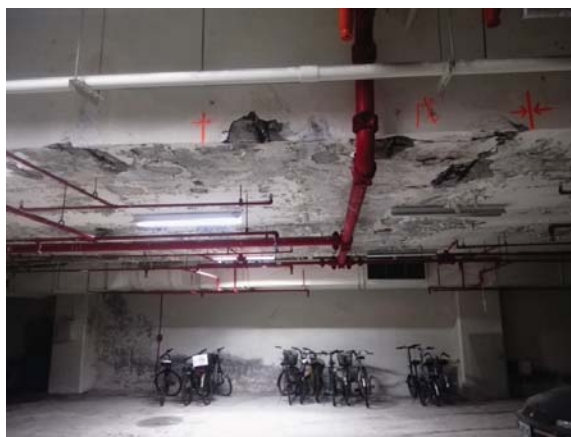
6 March 2017: B1/F of the loot storage prior to the repair
