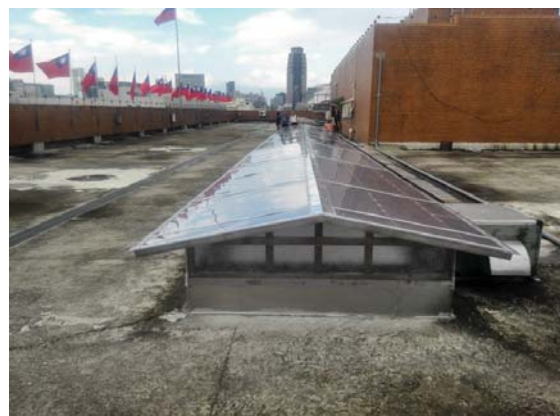
9 October 2018: roof skylight after the upgrade
