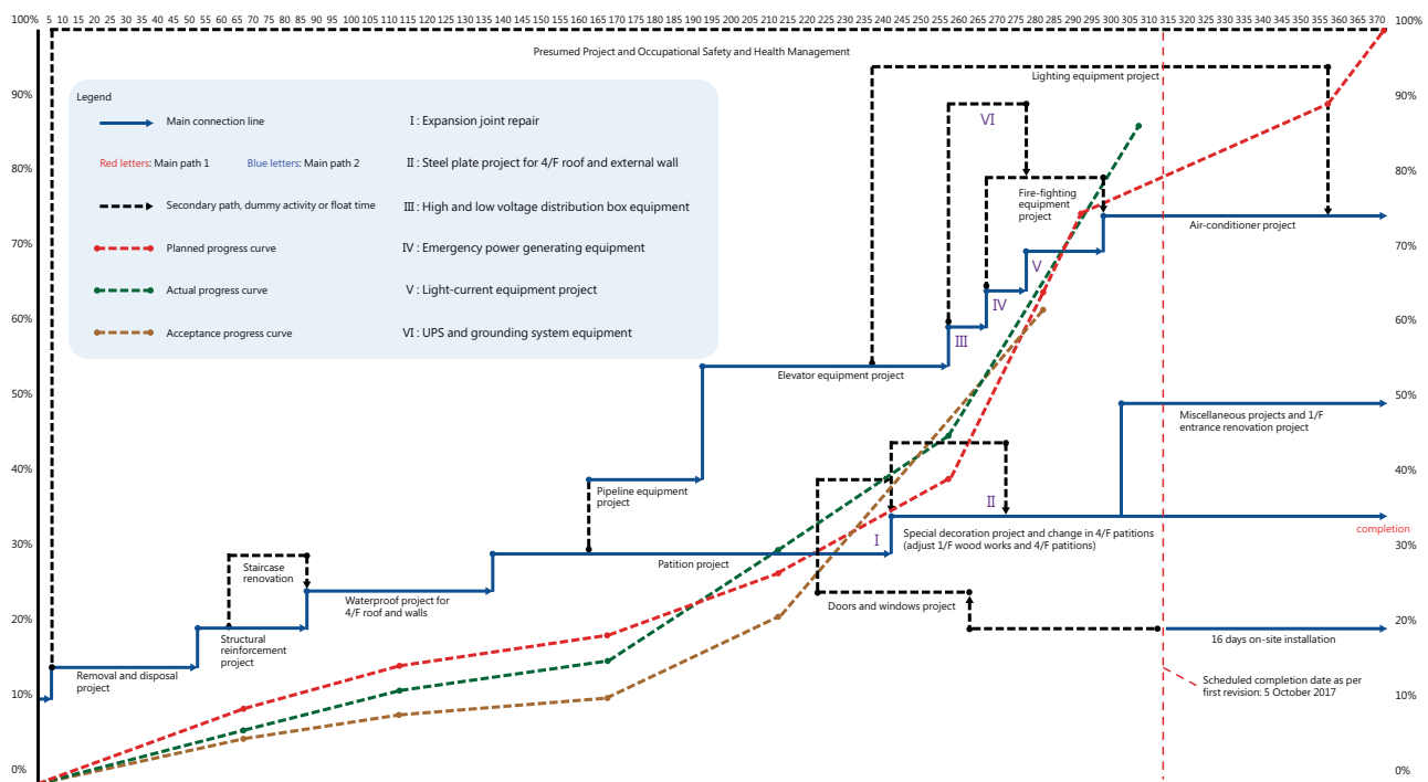
Project for the Offices in the Procurement Building of Taiwan Taipei District Court Prosecutors Office (in line with the second revision)
