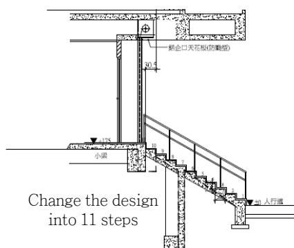
Reduce slope of the entrance stairs
