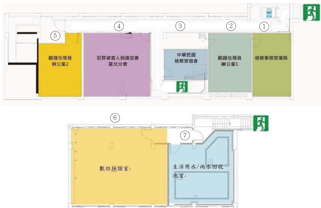
B1/F floor plan after the renovation
