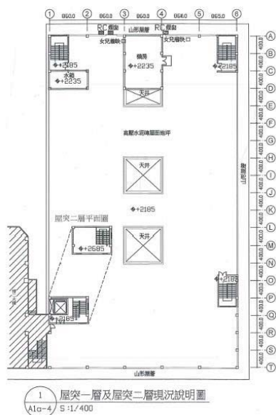
Pre-renovation plan(RF)
