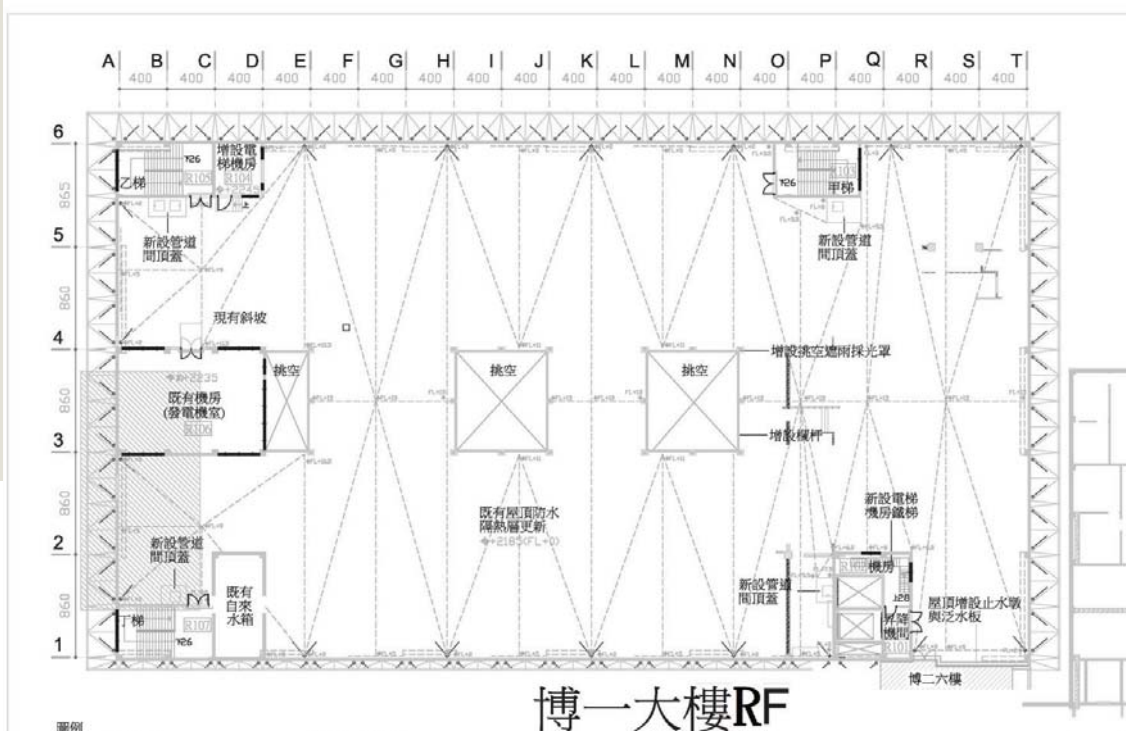
Layout after the renovation (RF)
