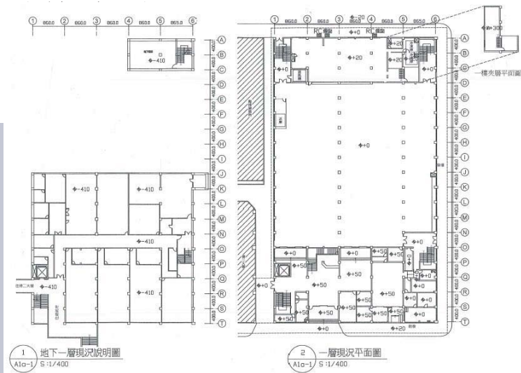
Pre-renovation plan(B1F, 1F)
