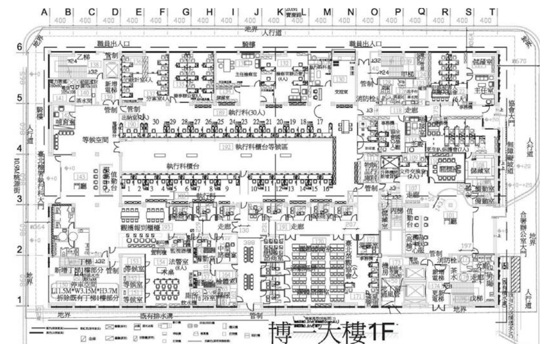
Layout after the renovation (1F)
